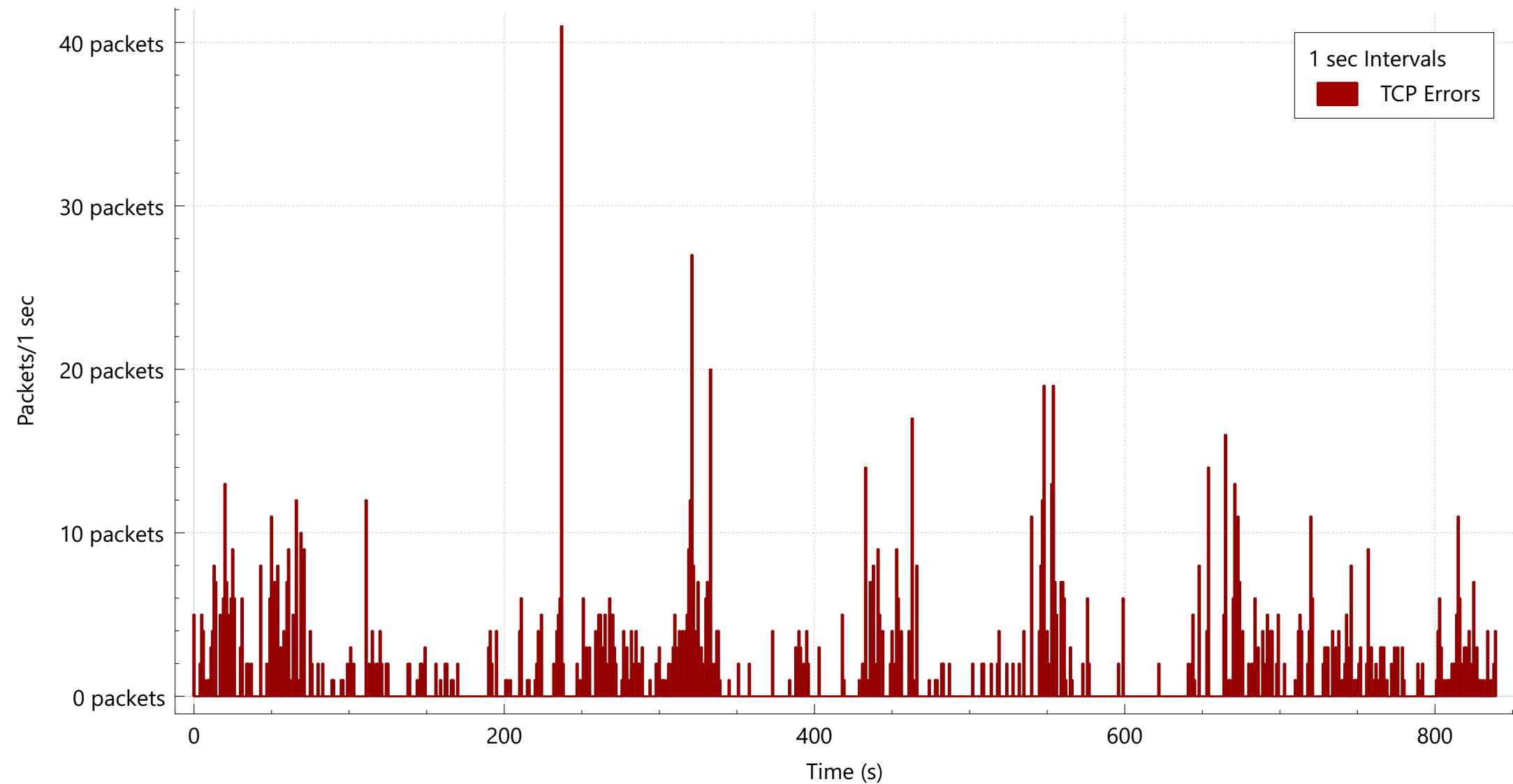
Wireshark I/O Graphs: Wireshark Network Analysis.pcapng
